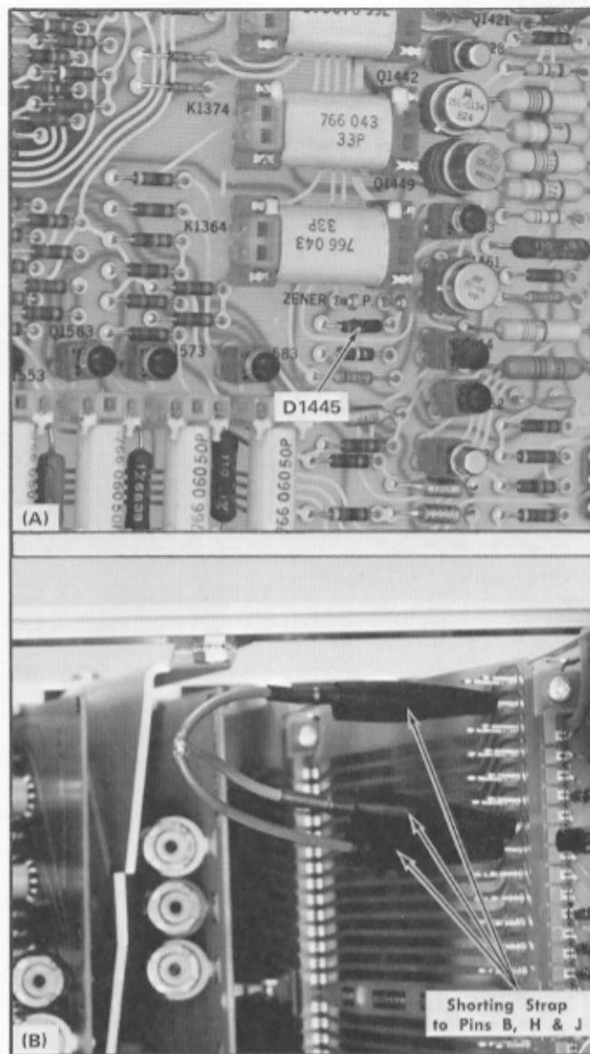
Fig. 7-6. Start Comparator circuit card with (A) location of D1445 and (B) special shorting strap connected.
