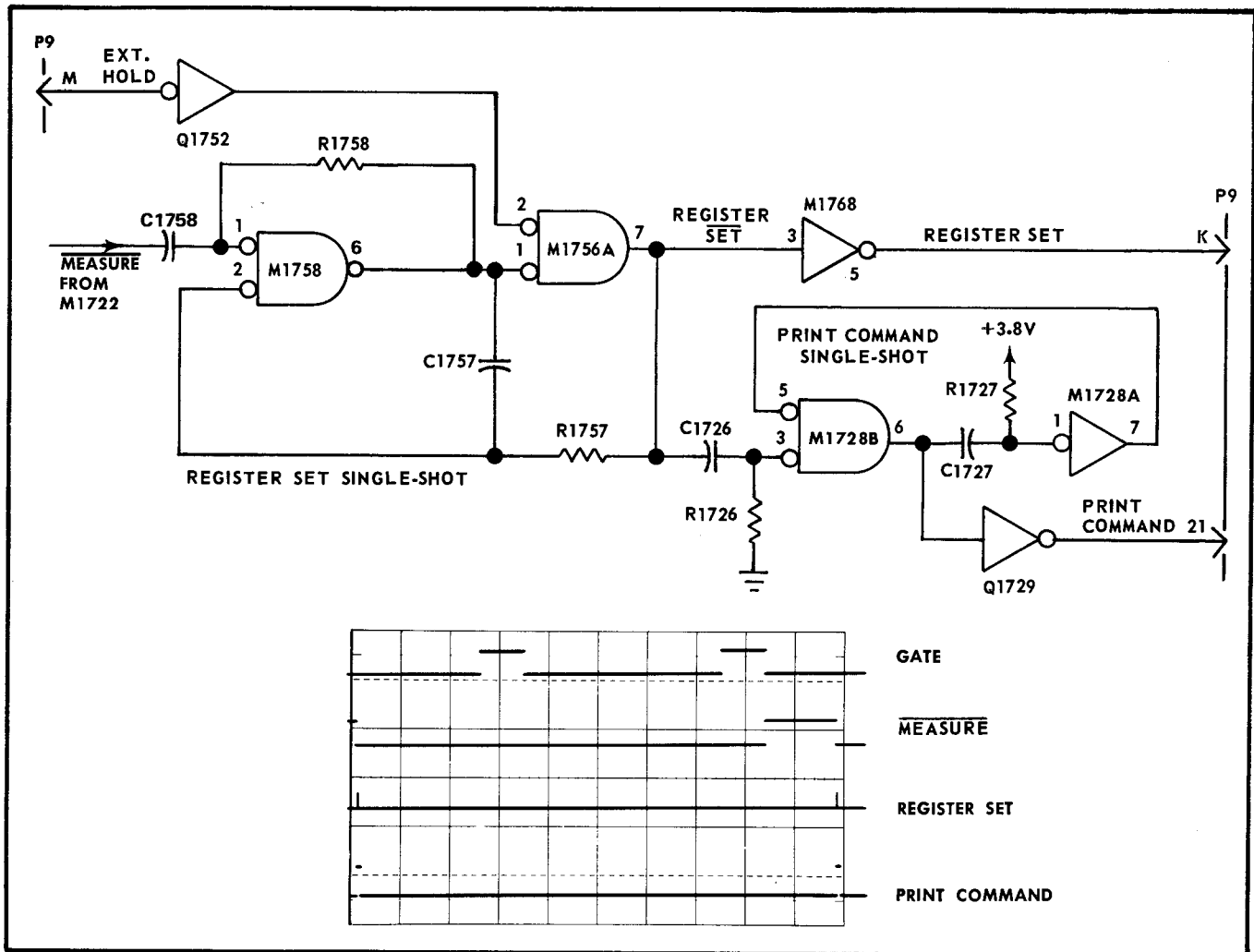
Fig. 4-22. REGISTER SET and PRINT COMMAND pulse generation (synchronizer models 1 and 2).
