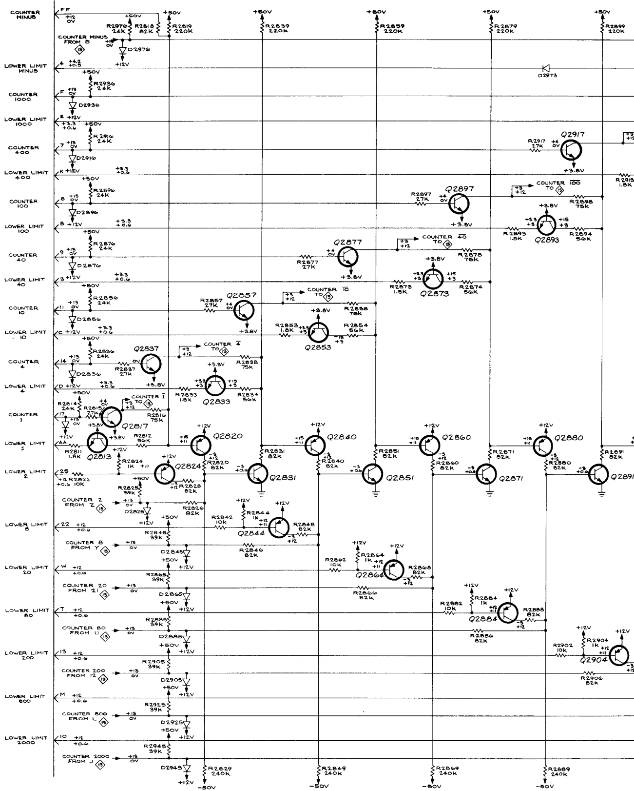
TYPE 230 DIGITAL UNIT
