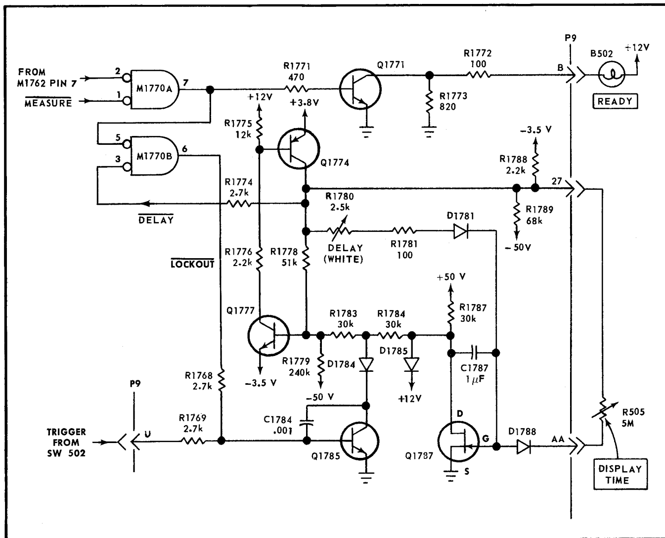
Fig. 4-18. \overline{\text{DELAY}} generation (synchronizer models 1 and 2).
